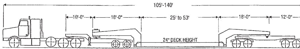
65 TON MULTI AXLE TRAILER
