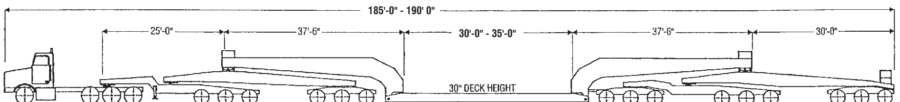
150 TON MULTI AXLE TRAILER
