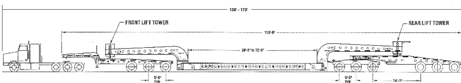
80 TON MULTI AXLE TRAILER
