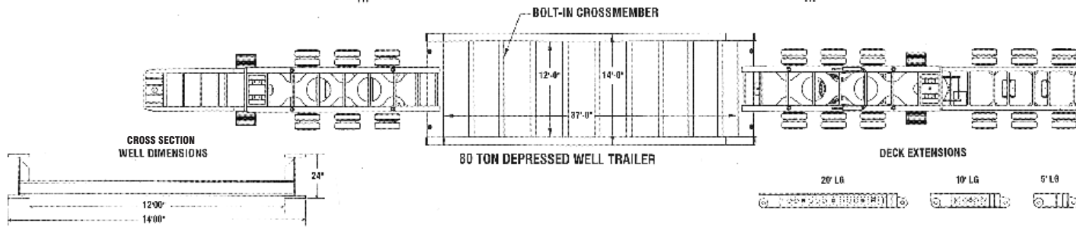
80 TON DEPRESSED WELL TRAILER
