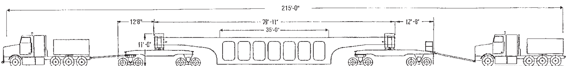
150 and 160 TON 18' WIDE DUAL LANE TRANSPORTER 16" AND 24" DECK HEIGHT
