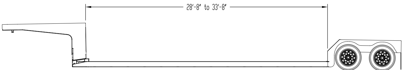
Lowboy Mini Deck Trailer Up to 30 Tons Capacity
