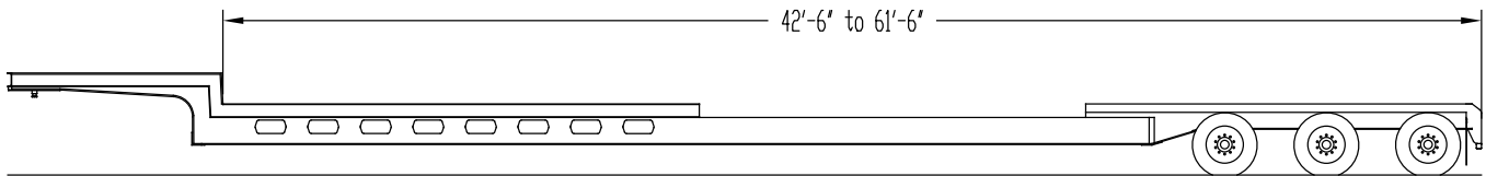
Extendable Drop Deck, Tri or Quad Axle Trailer Up to 50 Tons Capacity
