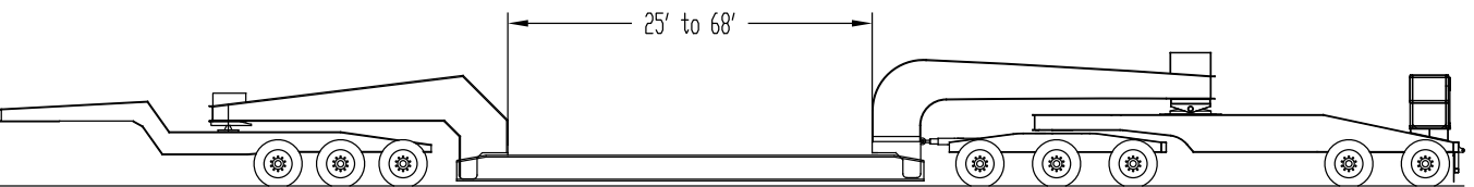
Flat and Depressed Well 11 Axle Trailer Up to 70 Tons Capacity
