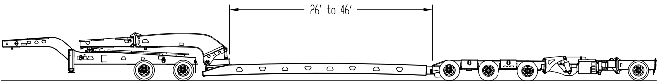
Extendable Lowboy Trailer Up to 50 Tons Capacity
